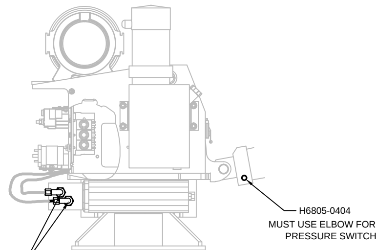
RIGHT SIDE
