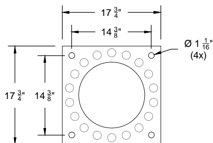
BASE MOUNTING DIMENSIONS (NOT TO SCALE)
